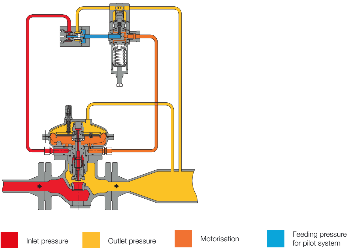
Figure 7 Dixi with fail to open pilot series 210
