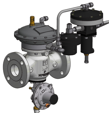
Figure 4 Dixi with LA slam shut valve
